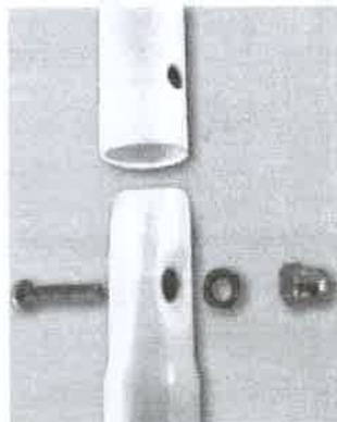
STEP III: Diagram of Connect bridge handrails with screws; washers and nuts
